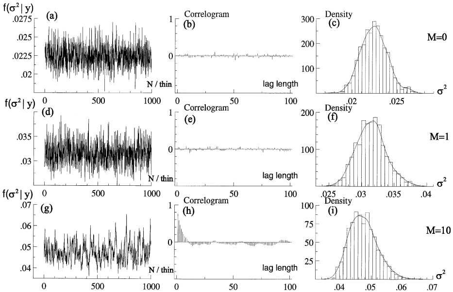
FIGURE 7.—Paths (a, d, g), correlograms (b, e, h), and histograms (c, f, i) for draws from \sigma^2 | y (true value 0.05). Top graph uses discretization M = 0 , middle graphs have M = 1 , and bottom graphs have M = 10 , \lambda = 3 . N = 10,000 with \text{thin} = 10 and \Delta^\dagger = 5 in all simulations.
