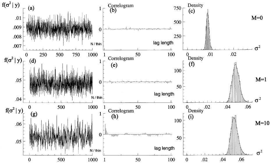
FIGURE 6.—Paths (a, d, g), correlograms (b, e, h), and histograms (c, f, i) for draws from \sigma^2 | y (true value 0.05). Top graph uses discretization M = 0 , middle graphs have M = 1 , and bottom graphs have M = 10 , \lambda = 3 . N = 10,000 with \text{thin} = 10 and \Delta^\dagger = 1 in all simulations.
