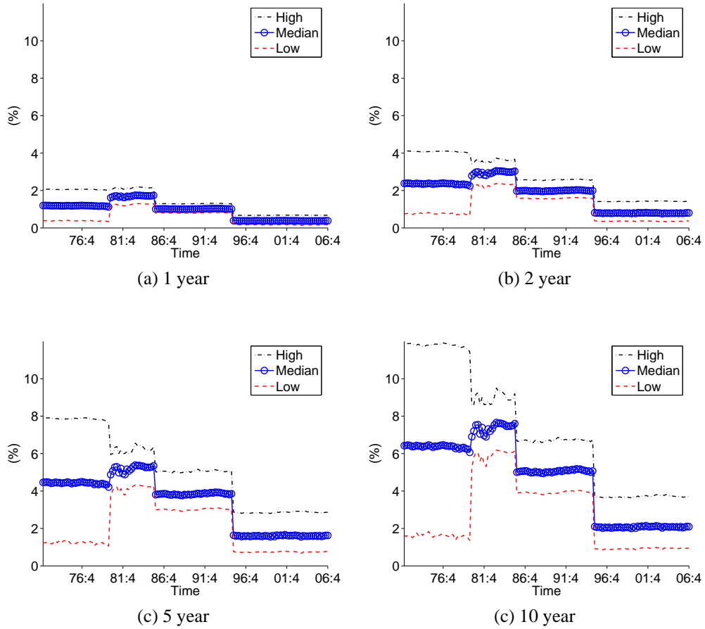
Figure 7: Model \mathcal{M}_3 : Term premium. The figure plots the 2.5%, 50% and 97.5% quantile of the posterior term premium based on 50,000 MCMC draws beyond a burn-in of 5,000 iterations.
